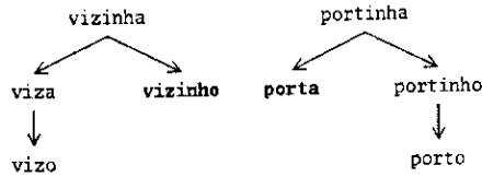
Figure 6: Branching search
