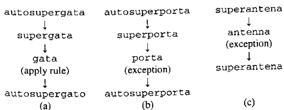
Figure 5: Prefix stripping
