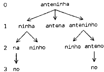
Figure 7: Lemmatizing anteninha
